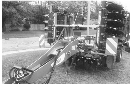
Farmet Softer 4.5 high spd. disc, demo model, 15'1" working width.
