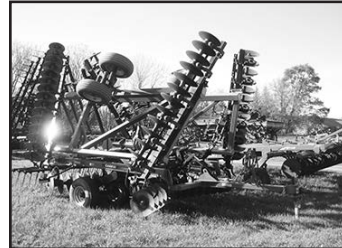
'12 Case IH 340 31' Tru tdm. disc., cushion gang, 22" 6.5 mm blades, hyd hitch, opt. gang brgs., 3-bar coil tine.
