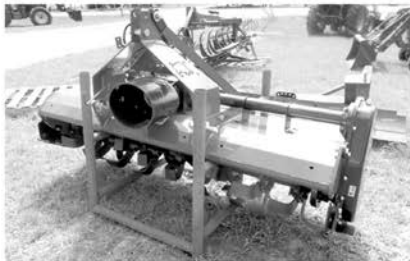
BUSH HOG TILLER RT72G 72", working width 70.5", 6 blades per flange, gear drivetrain, PTO w/slip clutch. $2,299
