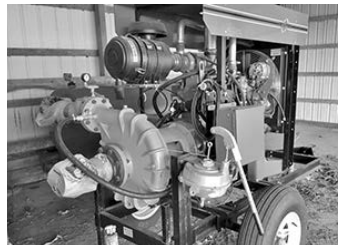
JOHN DEERE DIESEL/ BERKELEY PUMPING UNIT (used)
