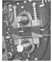
Heavy duty bearing houses with both rolls spring loaded.
